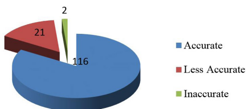
Figure 1. Translation Accuracy
